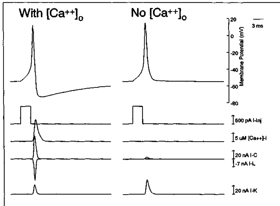
Figure 19. Addition of a \text{Ca}^{++} -activated \text{K}^+ current and a high-threshold \text{Ca}^{++} current helps to repolarize the membrane after each action potential in the modeled neuron. Reduction of I_c results in reduction of the hyperpolarization following the action potential, an increase in the duration of each action potential, and an increase in the amount of I_K activated.
