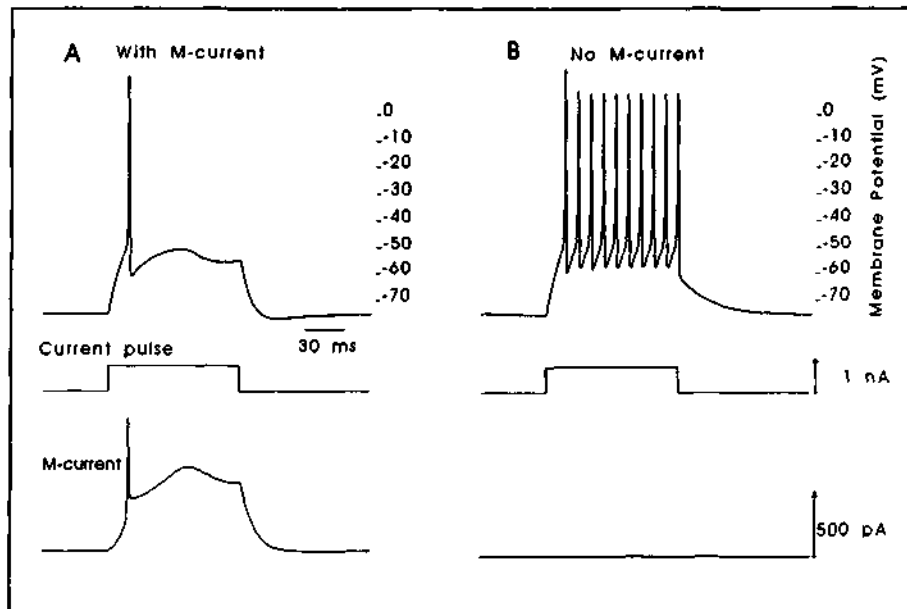
Figure 26. Depolarization activates a K^+ current known as the M-current, which subsequently prevents the generation of a train of action potentials in the model cell (A). Block of the M-current restores the ability of the cell to tonically fire (B).
