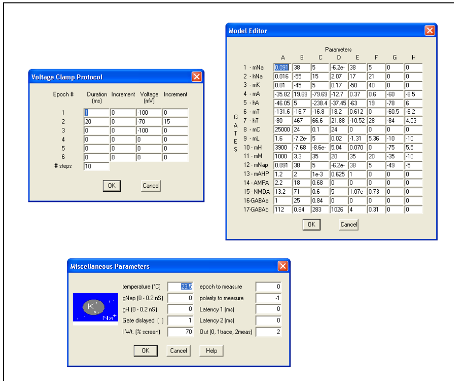
Figure 35. Options available under “Other” in VCWIN include the voltage step protocol (6 independent epochs to each step are available; typically only 3 are used), the constants for the equations used to model the ionic currents, the temperature, and amplitude of gNap and gH, as well as the epoch to make measures for plots.
