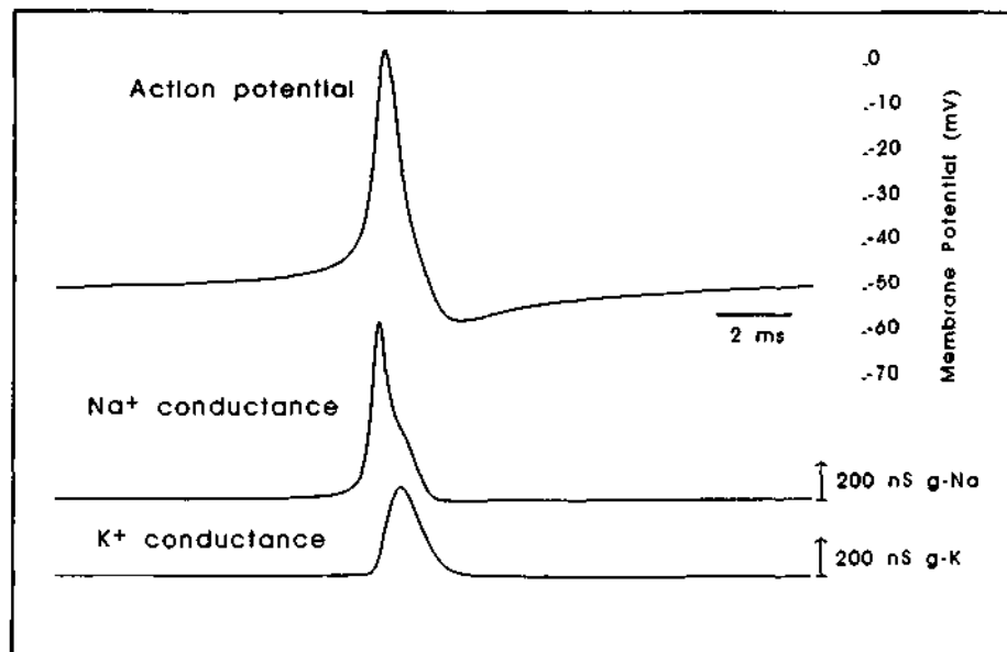
Figure 12. Amplitude and time course of the \text{Na}^+ and \text{K}^+ conductances ( g_{\text{Na}} , g_{\text{K}} ) during the generation of an action potential.
