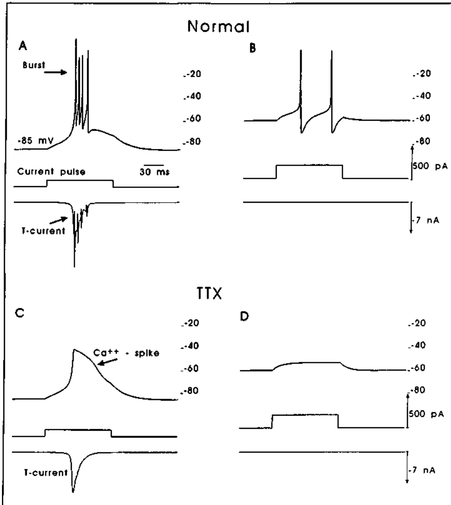
Figure 24. The transient Ca^{++} current generates burst discharges at hyperpolarized membrane potentials in the model cell. A , Injection of a depolarizing current pulse into this model "thalamic relay" cell results in a burst of action potentials. The burst is due to the activation of I_T . B , Depolarization of the cell to -60 mV inactivates the T-current and now the cell does not burst. C and D , Block of the Na^+ current with tetrodotoxin (TTX) reveals the underlying slow Ca^{++} spike and the lack of this Ca^{++} current when the cell is tonically depolarized to -60 mV.
