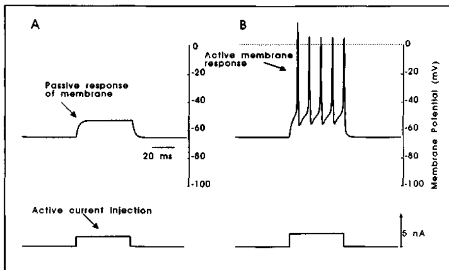
Figure 4. Passive and active membrane responses of model axon. A , Injection of a 1.5-nA current pulse (indicated in bottom trace ) results in only a passive response that results from the resistive/capacitive properties of the membrane. B , Injection of 2.0 nA of current results in a series of action potentials.
