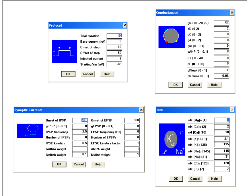
Figure 2. CCWIN menus. A, After starting CCWIN you can choose various pull-down menus such as File , Edit , Run , Parameters , Other , and Help . B, In the Parameters menu, you can change the Protocol, Conductances, Synaptic Currents, and Ions. The numbers in parentheses in the Conductances, Synaptic Currents, and Ions are the suggested values of these parameters. The items in Other menu are accessible only in Poweruser mode, see Appendix C, page 67.
