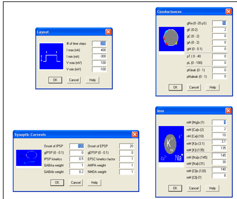
Figure 8. VCWIN menus. A , Starting the VCWIN program gives you access to pull-down menus: File , Edit , Run , Parameters , Other , and Help . B , In Parameters , you can adjust the Layout , Conductances , Synaptic Currents , and Ions . The numbers in parentheses in the Conductances , Synaptic Currents and Ions menus are the suggested values of these parameters. The items in Other menu are accessible only in Poweruser mode, see Appendix C, page 67.
